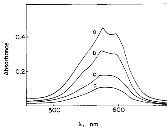
Figure 3. Shape of absorption band of p\text{-NH}_2\text{C}_6\text{H}_4\text{S}\cdot in ethyl acetate in the presence of both styrene ( 0.46\ \text{M} ) and oxygen ( p_{\text{O}_2} = 1.0 ): (a) 50\ \mu\text{s} , (b) 150\ \mu\text{s} , (c) 250\ \mu\text{s} , and (d) 500\ \mu\text{s} after flash.
