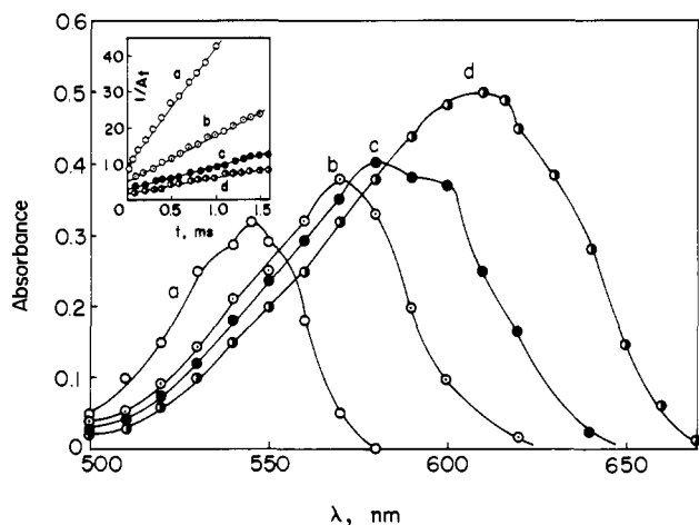
Figure 1. Solvent effect on the absorption band of p\text{-NH}_2\text{C}_6\text{H}_4\text{S}\cdot ; transient absorption spectra observed at 30\ \mu\text{s} after the flash photolysis of (p\text{-NH}_2\text{C}_6\text{H}_4)_2\text{S}_2 ( 2.0 \times 10^{-5}\ \text{M} ) in (a) cyclohexane, (b) toluene, (c) tetrahydrofuran, and (d) dimethyl sulfoxide at 23\ ^\circ\text{C} . Insert: Second-order plots for decays of the transient absorption bands at each peak. A_t refers absorbance at time t .
