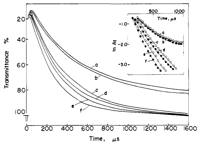
Figure 2. Oxygen concentration effect on the decay curves of p\text{-NH}_2\text{C}_6\text{H}_4\text{S}\cdot in the presence of styrene in ethyl acetate (at absorption peak 578\ \text{nm} ): (a and b) in degassed solution without styrene (a) and with styrene (b) ( 0.46\ \text{M} ); (c-f) variation in partial pressure of oxygen ( p_{\text{O}_2} ) in the presence of styrene ( 0.46\ \text{M} ), (c) p_{\text{O}_2} = 0.07 , (d) p_{\text{O}_2} = 0.11 , (e) p_{\text{O}_2} = 0.18 , and (f) p_{\text{O}_2} = 1.0 . Insert: First-order plots of the decay curves above.
